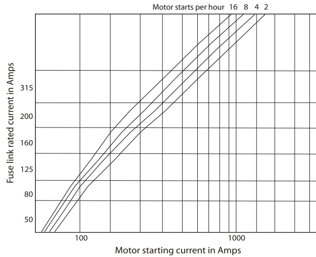
Fuse Selection Chart for Motor Protection with run-up time not exceeding 30 seconds
