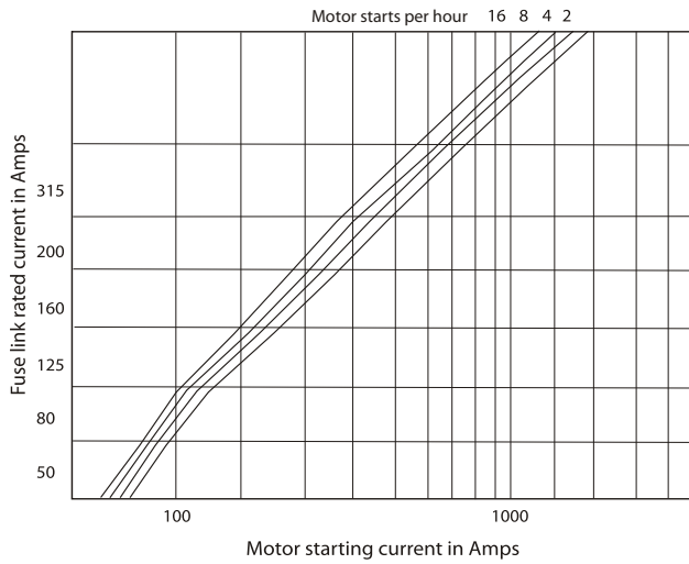
Fuse Selection Chart for Motor Protection with run-up time not exceeding 5 seconds
