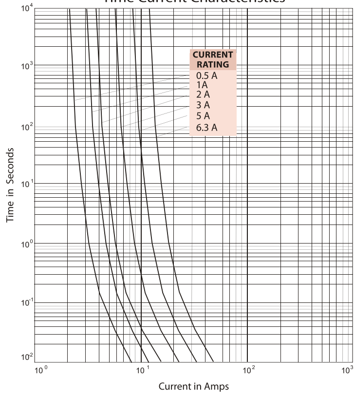
Time Current Characteristics
