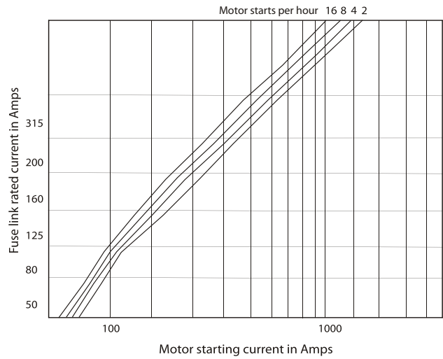
Fuse Selection Chart for Motor Protection with run-up time not exceeding 15 seconds
