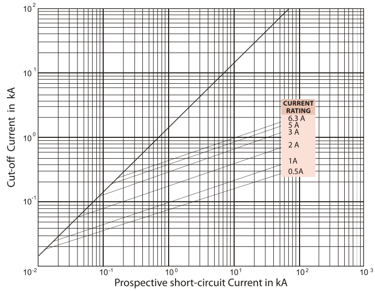
Cut-off Current characteristics
